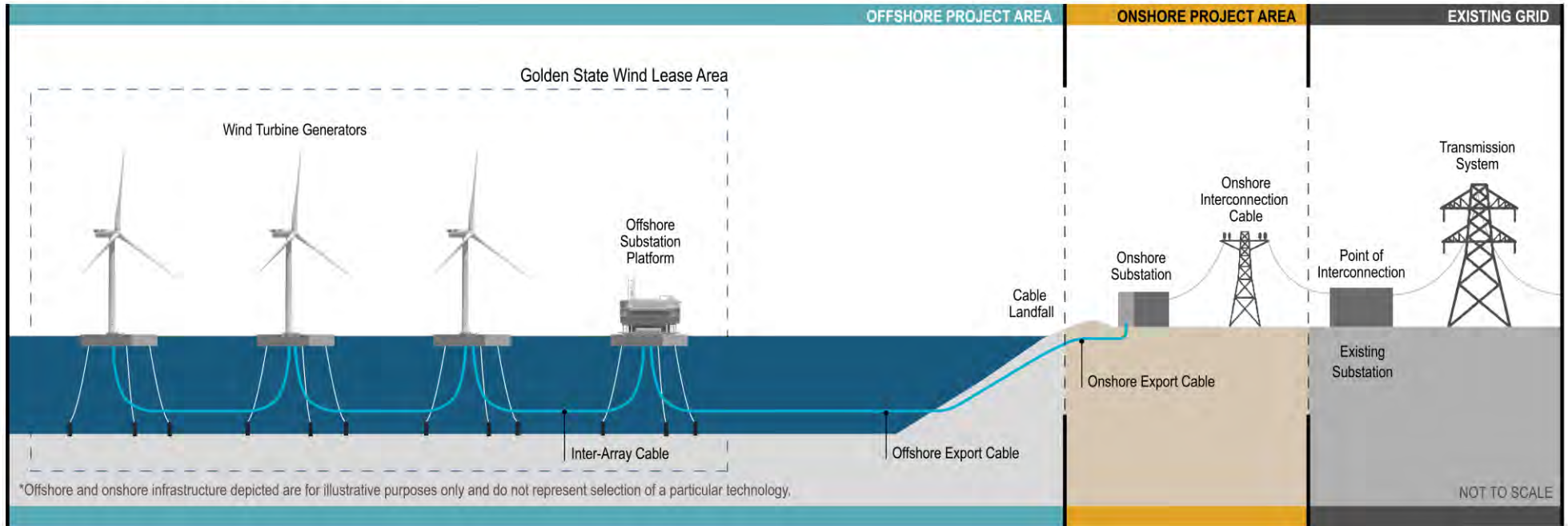
Figure 2. Project Schematic
